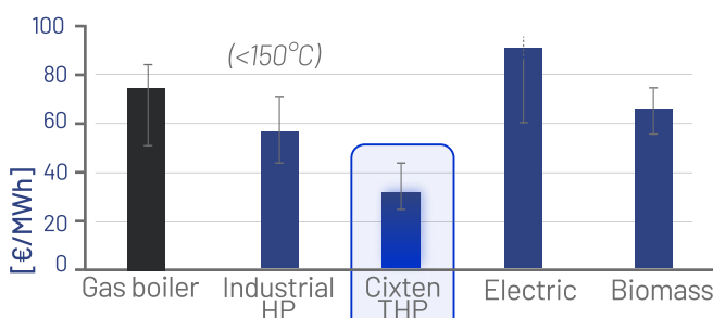
LCOH of industrial heat production solutions (€/MWh) :
